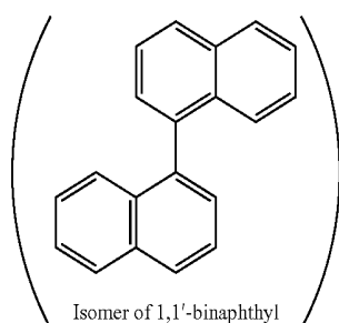
Isomer of 1,1'-binaphthyl
