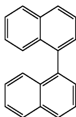
1,1'-binaphthyl
